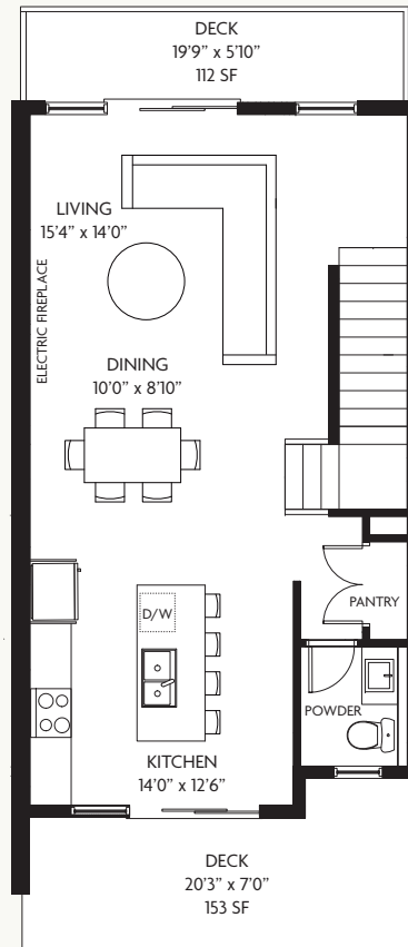
LEVEL 2 674 SF
