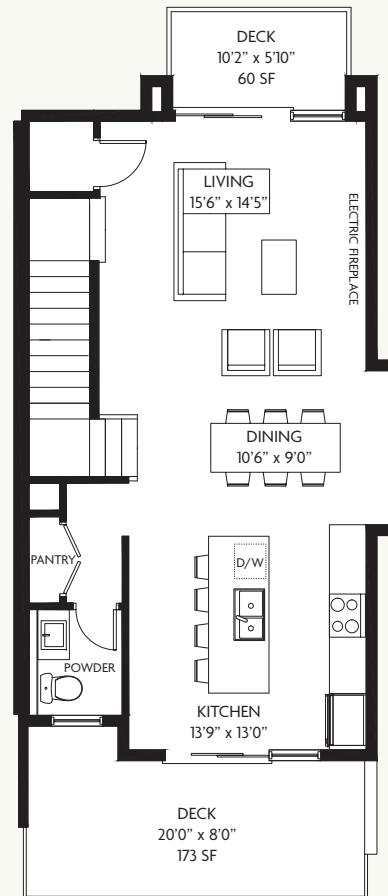
LEVEL 2 712 SF
